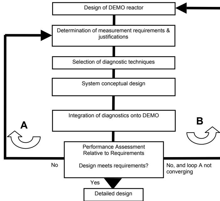
Figure 1. Scheme of integration of measurement and control requirements into a DEMO device design [4].
